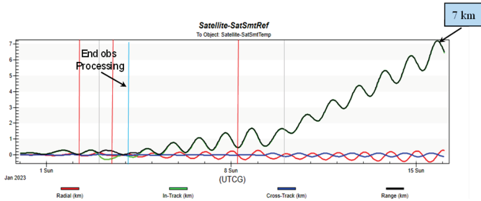
Fig. 11 - Ops Cadence Position Uncertainty (Optical Obs): Positional uncertainty where obs processing ended 5 Jan, 0154. The position uncertainty is about 7 km at the end of the interval.
