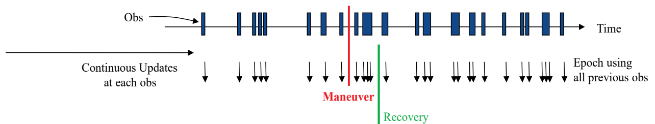
Fig. 7 - Comparison of BLS and EKF approaches in the Presence of a Maneuver. The BLS OD averages observations over a fit span, this lengthening the amount of time until full recovery can be made. The EKF, by processing each observation sequentially, reduces the time until recovery.
