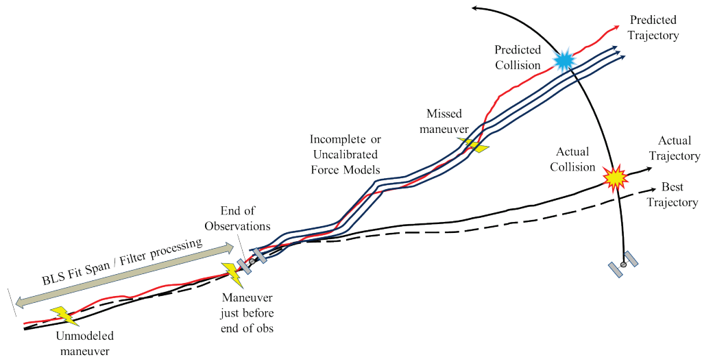
Fig. 1 - Conditions that degrade SSA. There are many conditions that can arise that prevent the accurate determination of the satellite state. Both the orbit determination and orbit prediction must be accurate. The goal is to minimize the difference of the actual and best estimated trajectories.
