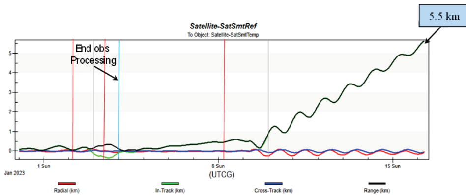
Fig. 12 - Ops Cadence Position Uncertainty (Optical Obs): Positional uncertainty where obs processing ended 5 Jan, 0636. The additional data gives about a 2 km improvement over the 10-day prediction interval from the case ending at 5 Jan, 0154.
